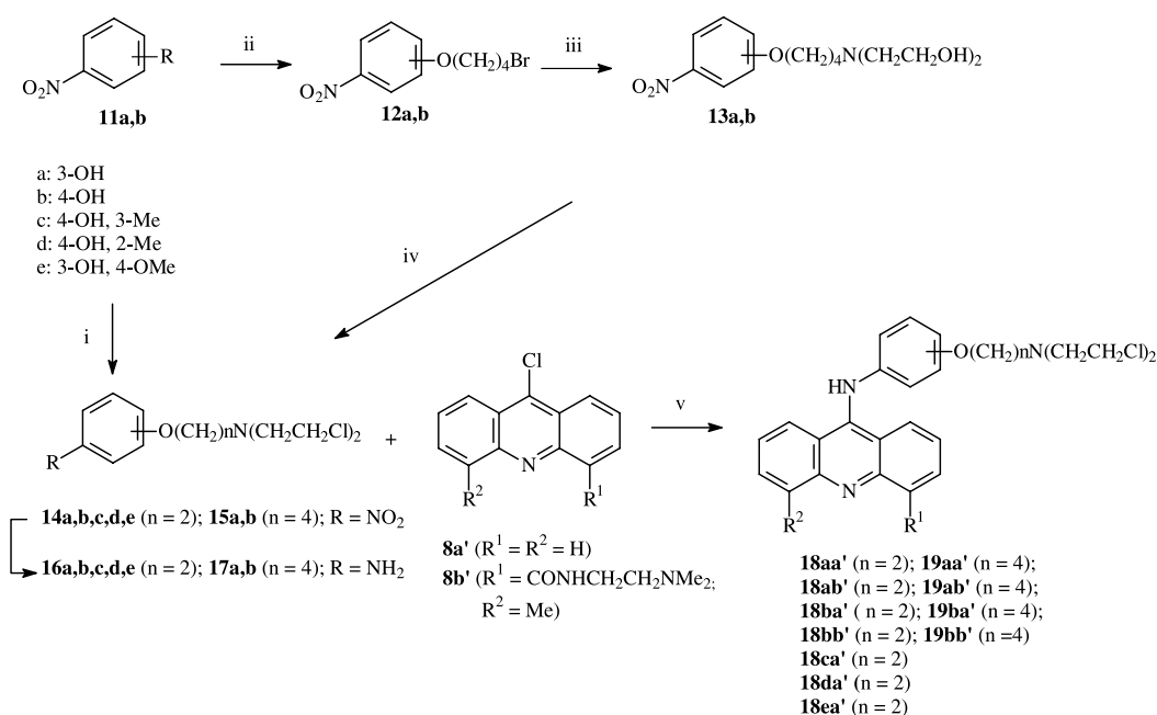
Scheme 2. Reagents and conditions: (i) Tris(2-chloroethyl)amine hydrochloride/K 2 CO 3 /KF/acetone, reflux; (ii) Br(CH 2 ) 4 Br/K 2 CO 3 /acetone, reflux; (iii) NH(CH 2 CH 2 OH) 2 /DMF, 110 °C; (iv) MeSO 2 Cl/Et 3 N, 0 °C to rt, 2 days; (v) CHCl 3 /EtOH/concd HCl (catalytic amount).
