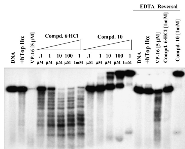
Figure 3. Topoisomerase II-mediated DNA cleavage by AHMA·HCl ( 6 ), compound 10 and VP-16.
