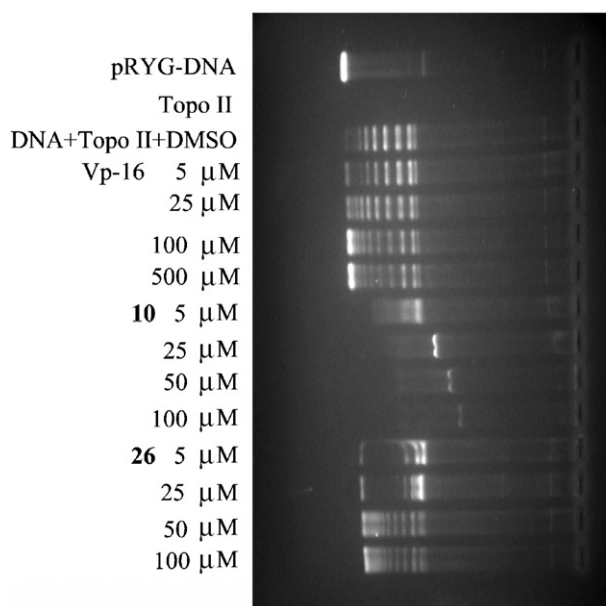
Figure 2. Comparison of Topo II-mediated relaxation of pRYG–DNA induced by VP-16, compound 10 and AHMA– tert -butylcarbamate ( 26 ). These agents inhibited DNA relaxation. However, compound 10 bind tightly to DNA.
