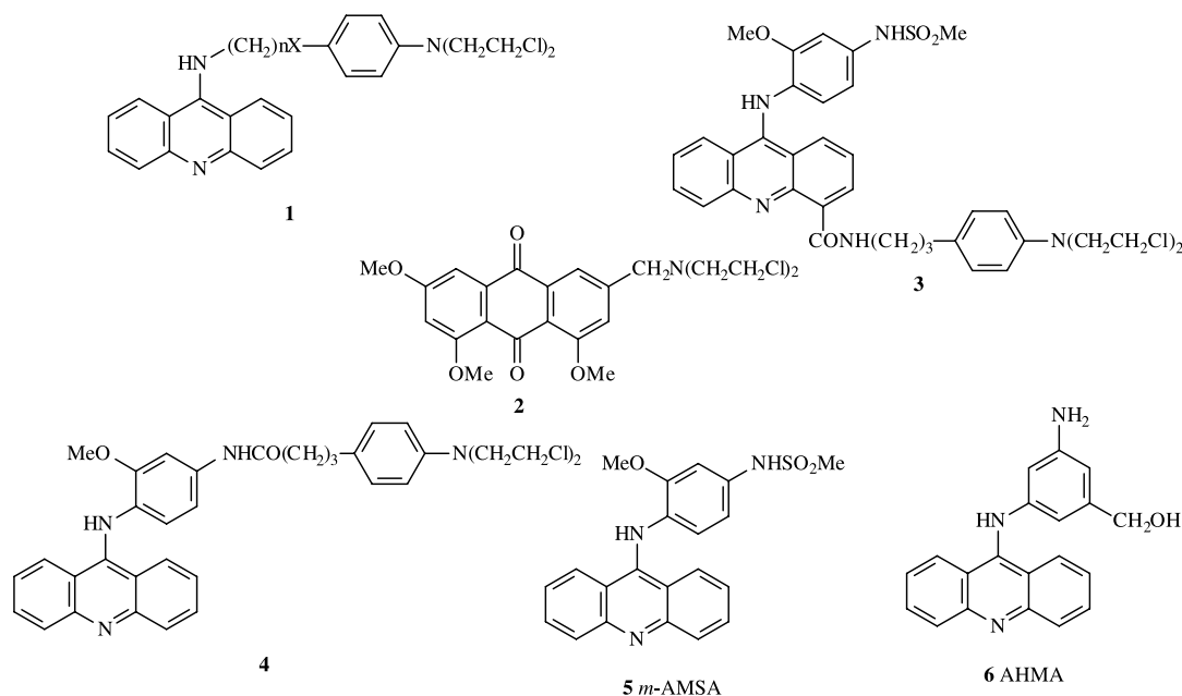
Chart 1. Structures of N-Mustard analogues and AHMA.
