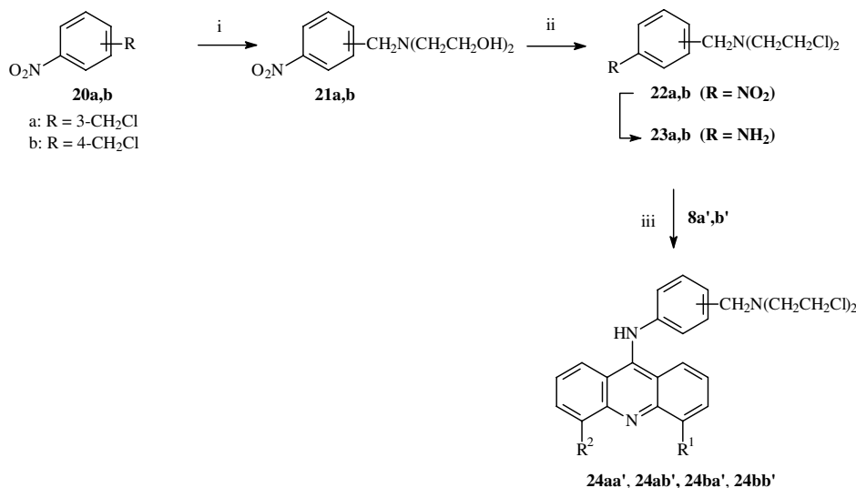
Scheme 3. Reagents and conditions: (i) NH(CH 2 CH 2 OH) 2 , 120 °C; (ii) MeSO 2 Cl/Et 3 N, 0 °C to rt, 2 days; (iii) CHCl 3 /EtOH/concd HCl (catalytic amount).
